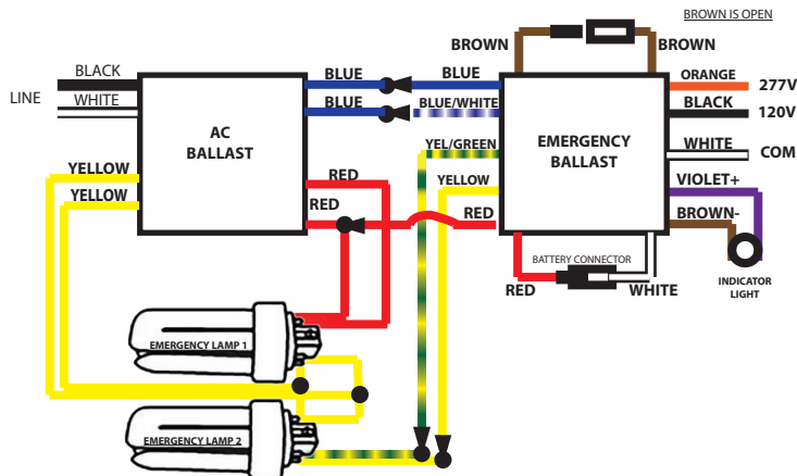
TWO LAMP PROGRAMMED START BALLAST Two Emergency Lamps
