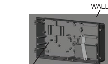
DRILL THROUGH THE HOLE; LOCK THE BASE ONTO THE WALL FIGURE 1
