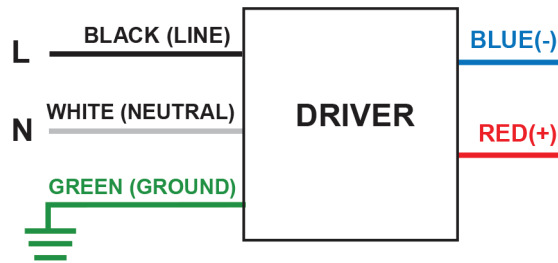
WIRING DIAGRAM
