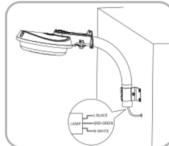
3. Connect wires per wiring diagram below.
