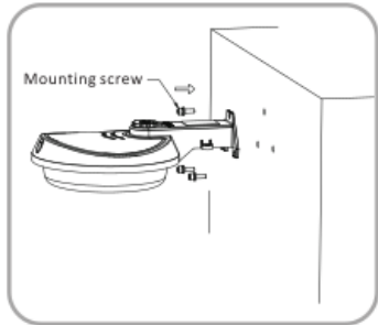
1. Mount the fixture to the wall via the mounting screws.
