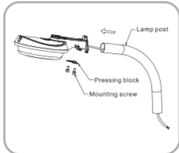
1. Run wiring through arm attachment and lock the pressing block
